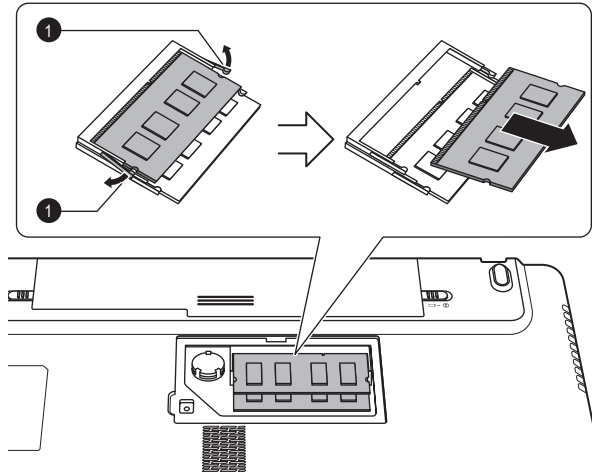
Figure 3-12 Removing the memory module (Satellite L770/L775/L770D/L775D/satellite Pro L770/L775/L770D/L775D)
